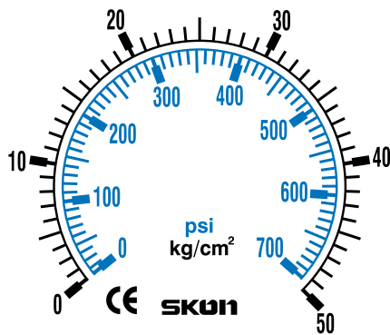
PSI and kg/cm 2 Size: 75mm acc.±1.5%
