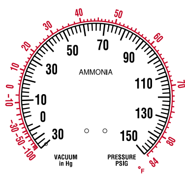
in Hg and Psi acc. \pm 1.5\% Ammonia Gauge
