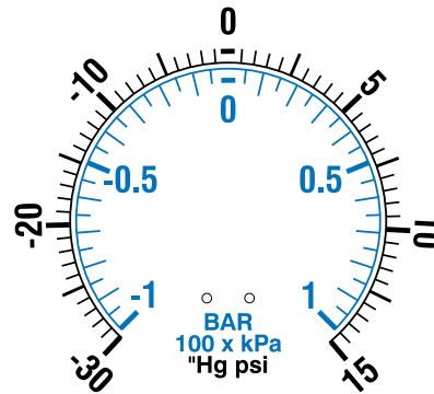
BAR and Psi acc. \pm 1.5\% Compound Pressure Gauge
