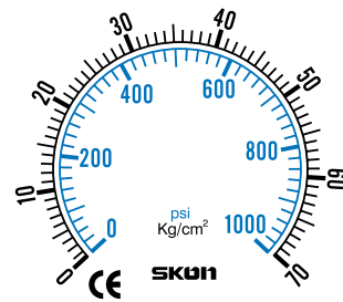
PSI and kg/cm 2 Size: 63mm acc.±1.5%
