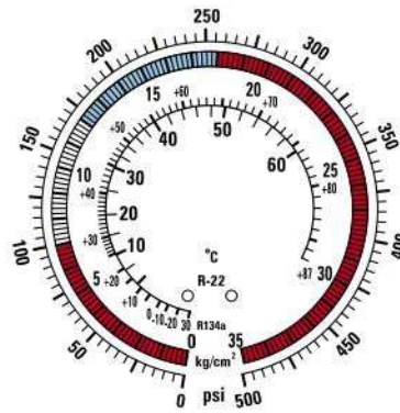
PSI and kg/cm 2 Freon Gauge
