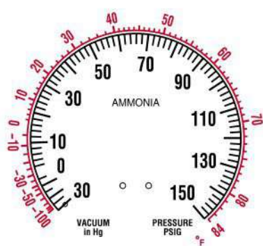
inHg and Psi Ammonia Gauge
